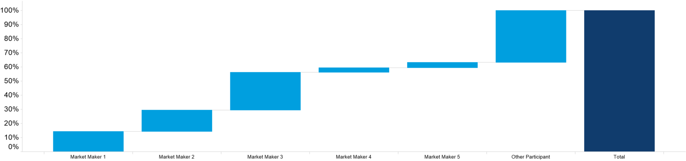
Market Maker Concentration (Sell Side) - January 2023
