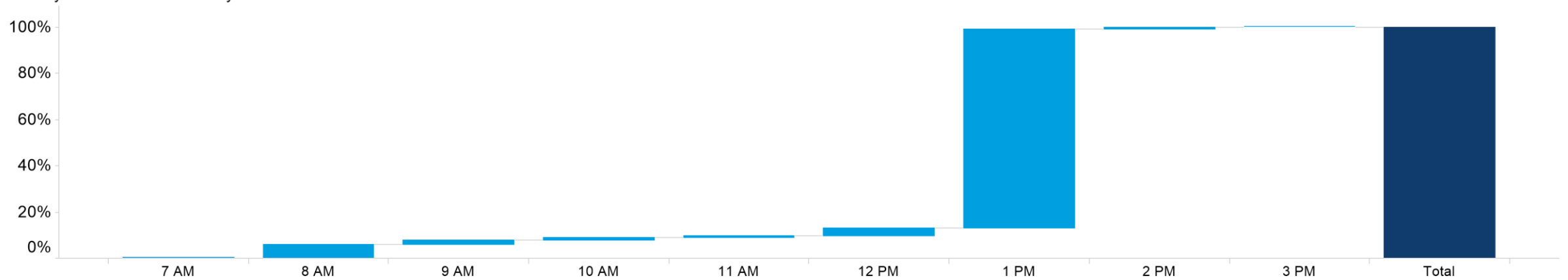
Time of Day Execution All - January 2023
