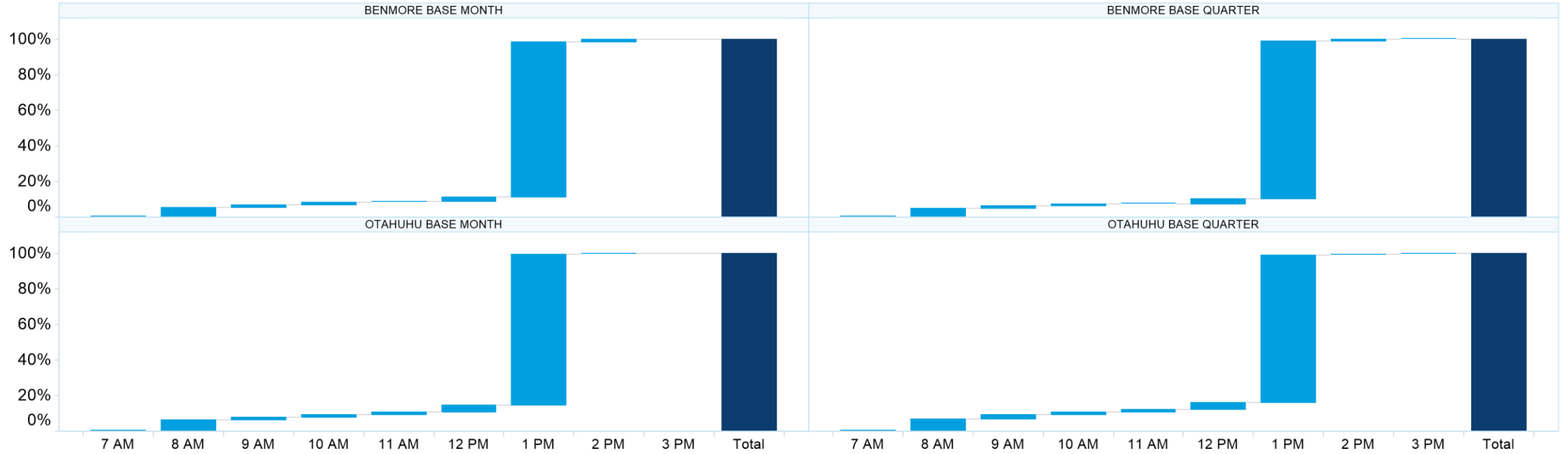
Time of Day Execution All - January 2023
